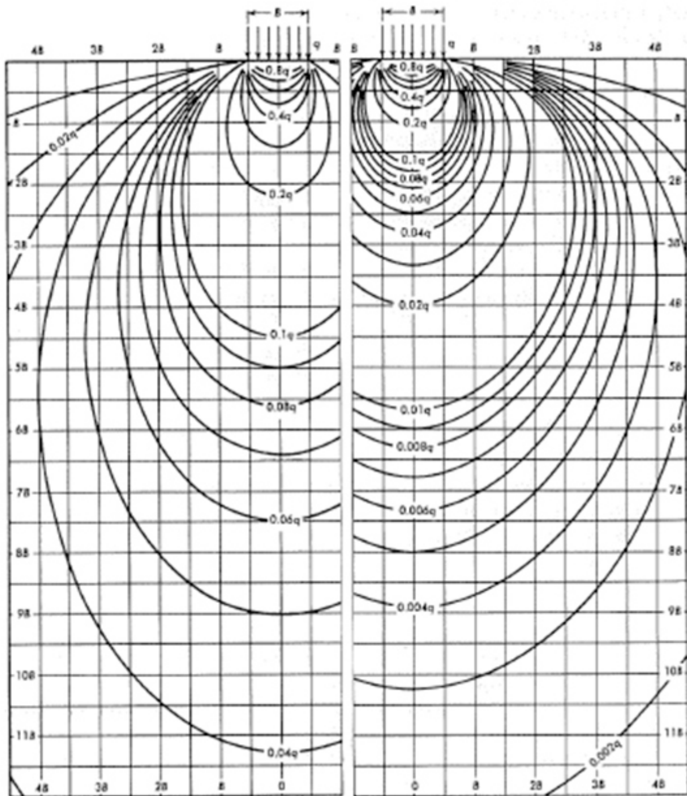
a. Infinitely long foundation
